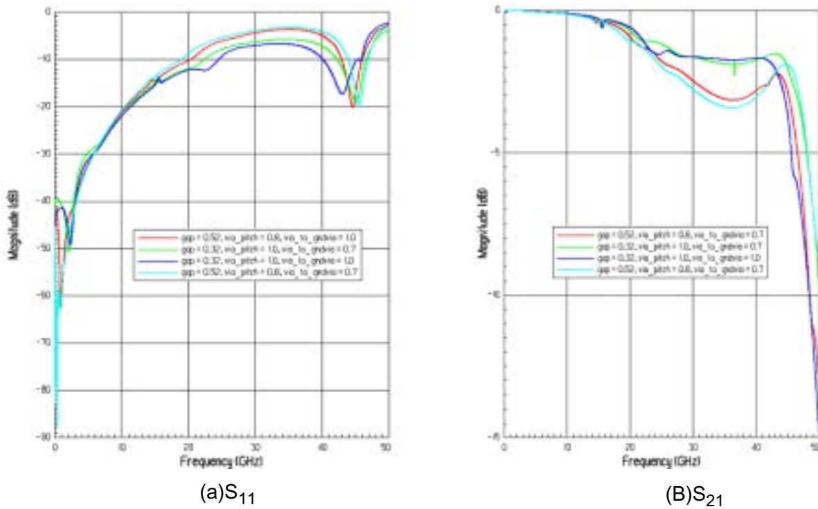
Figure 66 Extracted s-parameters for the four alternative GSSG via
